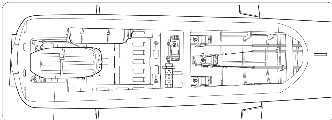
Fuel Tank
